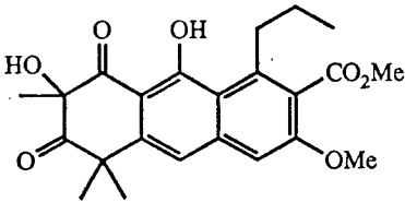
2-hydroxygarvin A
