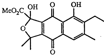
annulin A
