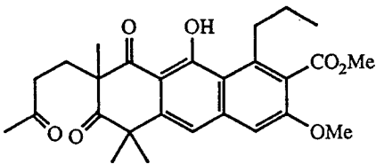
garvalone A
