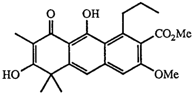
garvin A
