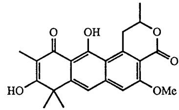
garvin B
