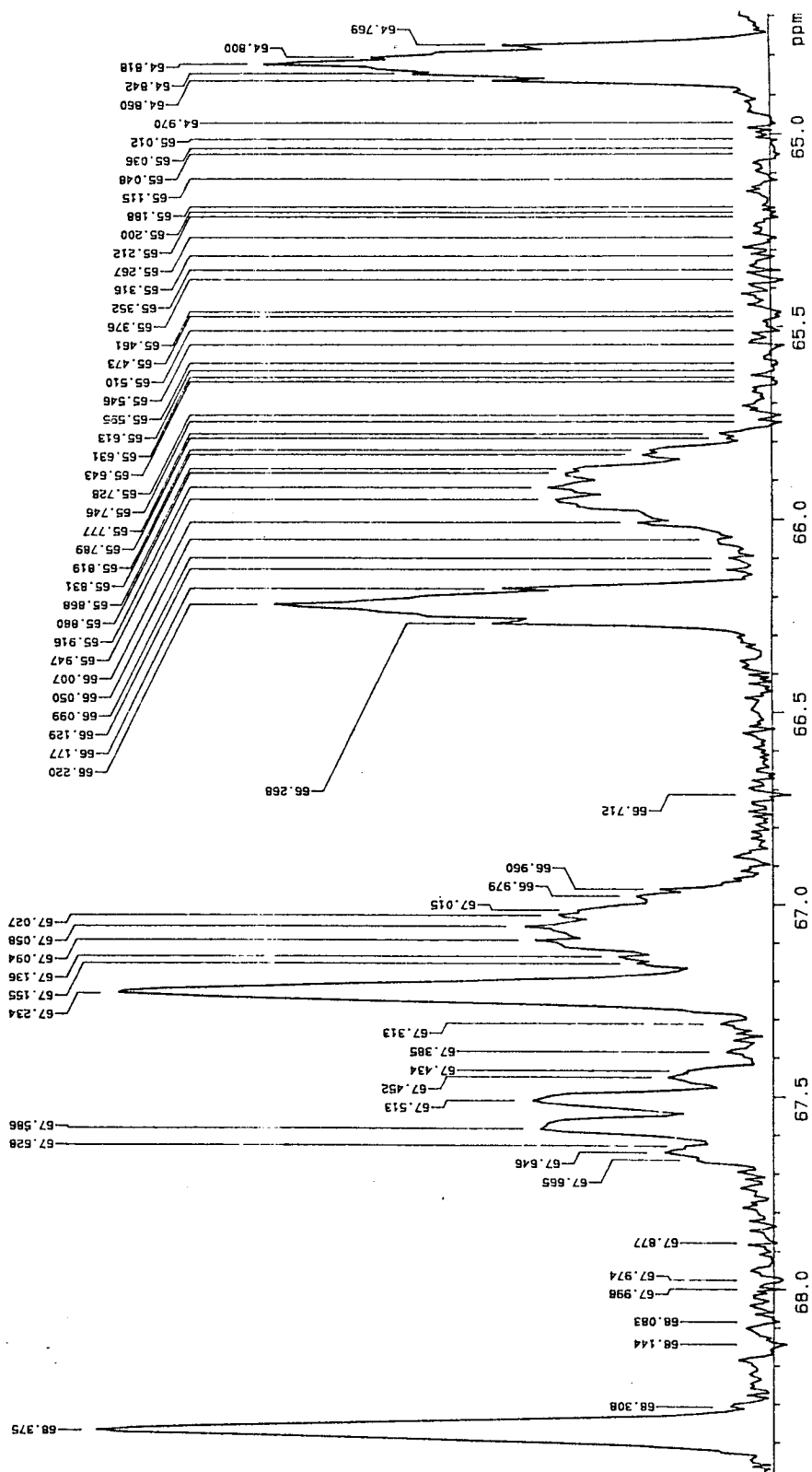
Fig. 3-27. Proton coupled carbon NMR spectrum of polyhydroxy steroids (60 - 80 ppm region).
