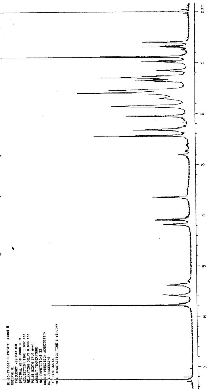
Fig. 5-9. Proton NMR spectrum of compound 91-10-2.
