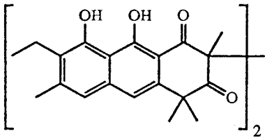
( Garveia annulata )
