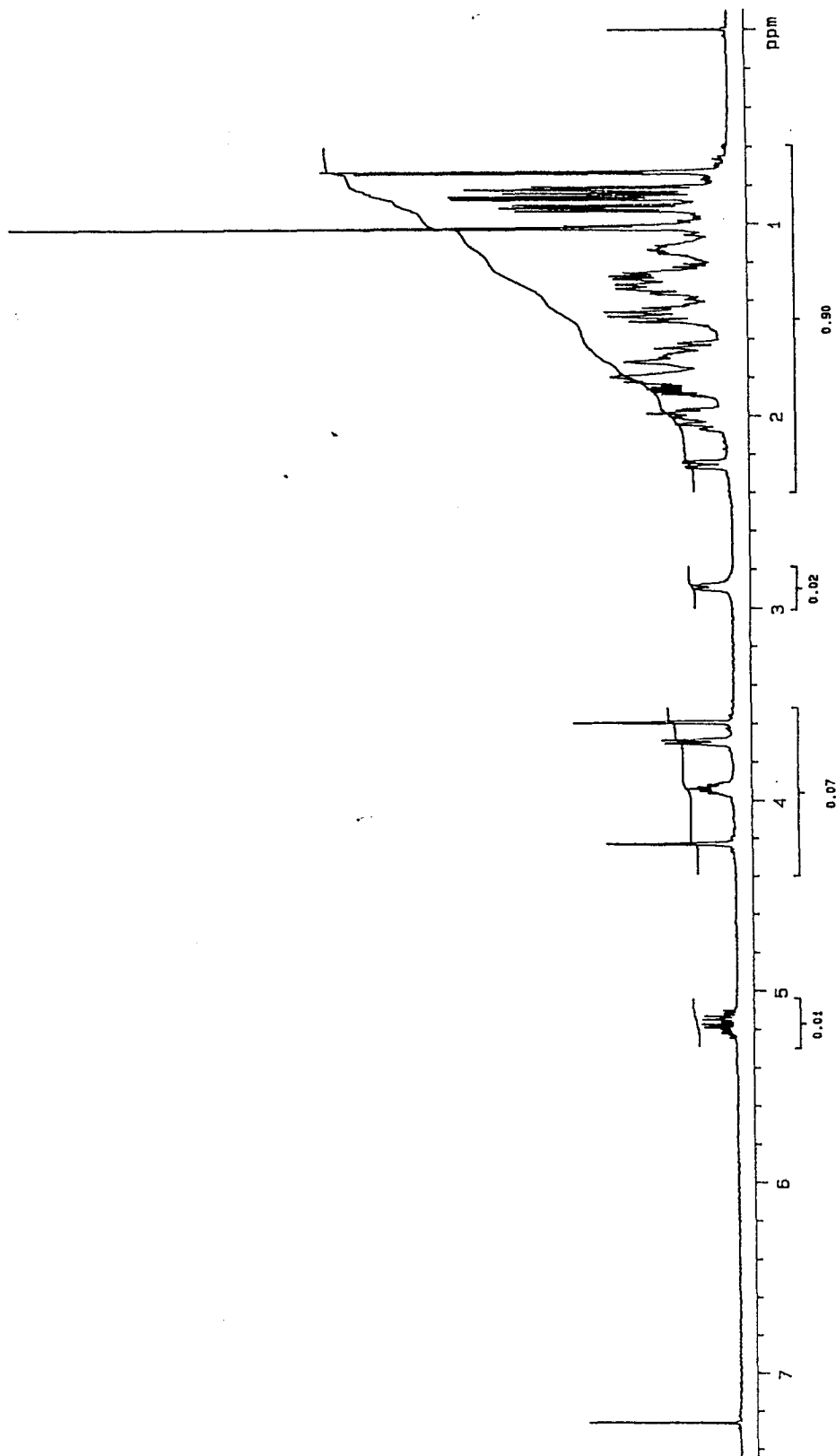
Fig. 3-23. Proton NMR spectrum of mixture of polyhydroxy steroids isolated from the gorgonian Acabaria undulata .
