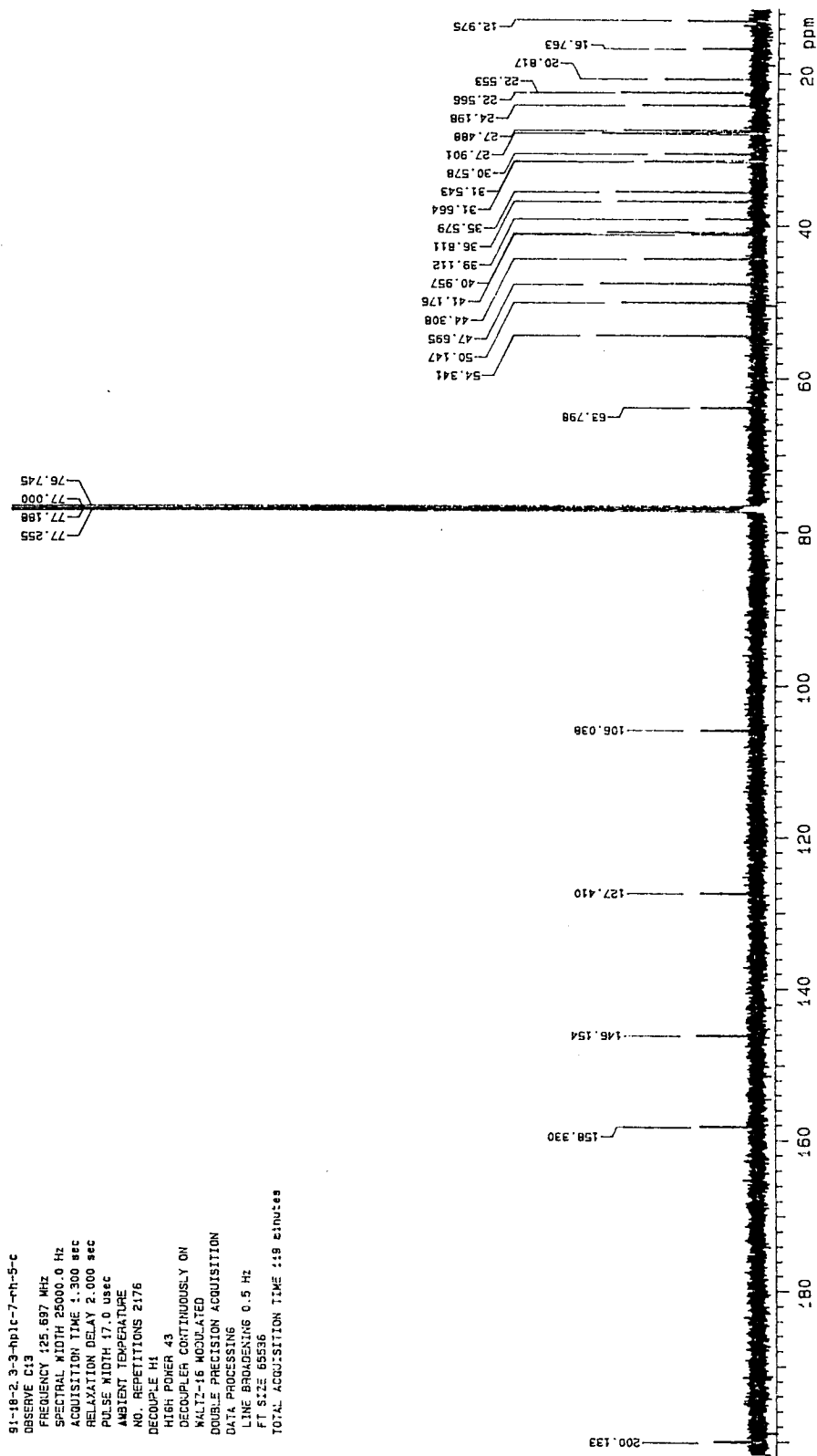
Fig. 4-12. Carbon NMR spectrum of compound 91-18-4.
