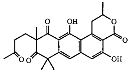
garvalone B
