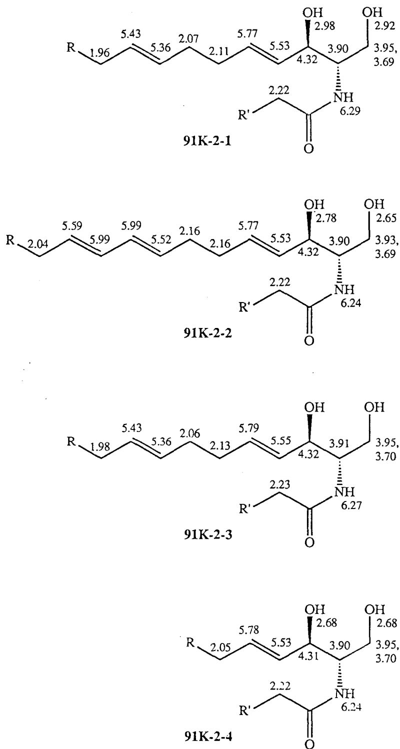
Fig. 3-10. Partial structures and ^1\text{H} NMR assignments for compounds 91K-2-1 ~ -4.
