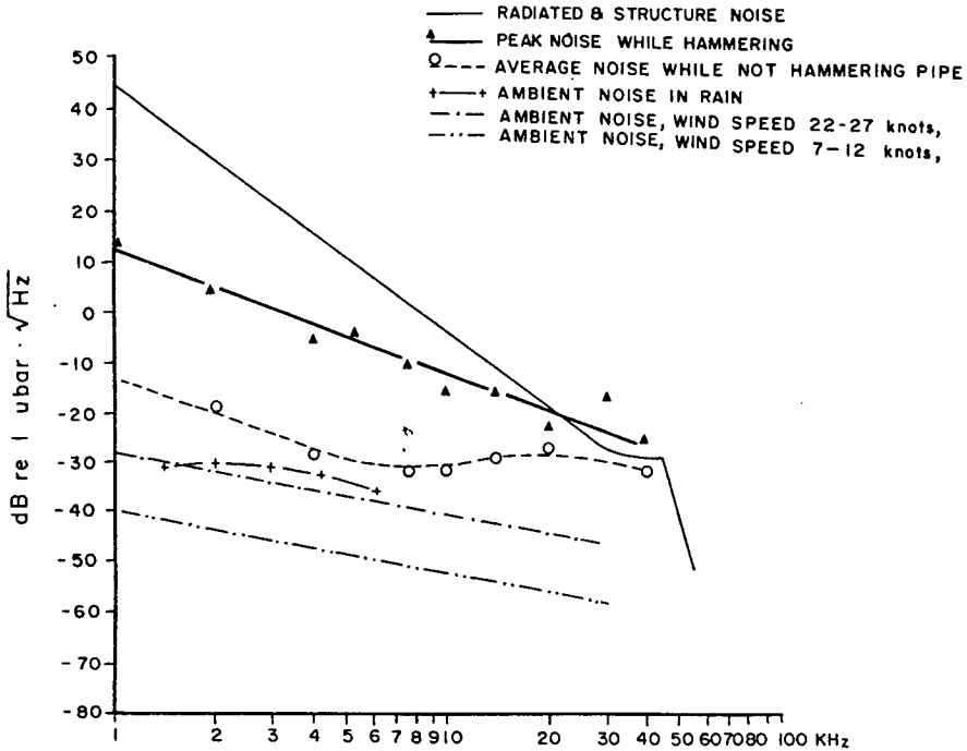
Fig. 3. Ambient noise in man-made and natural environments.
